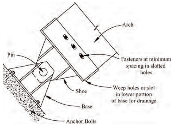
Figure C1.1.1 (a) Typical arch base with thru-bolt and (b) arch base with true hinge.
