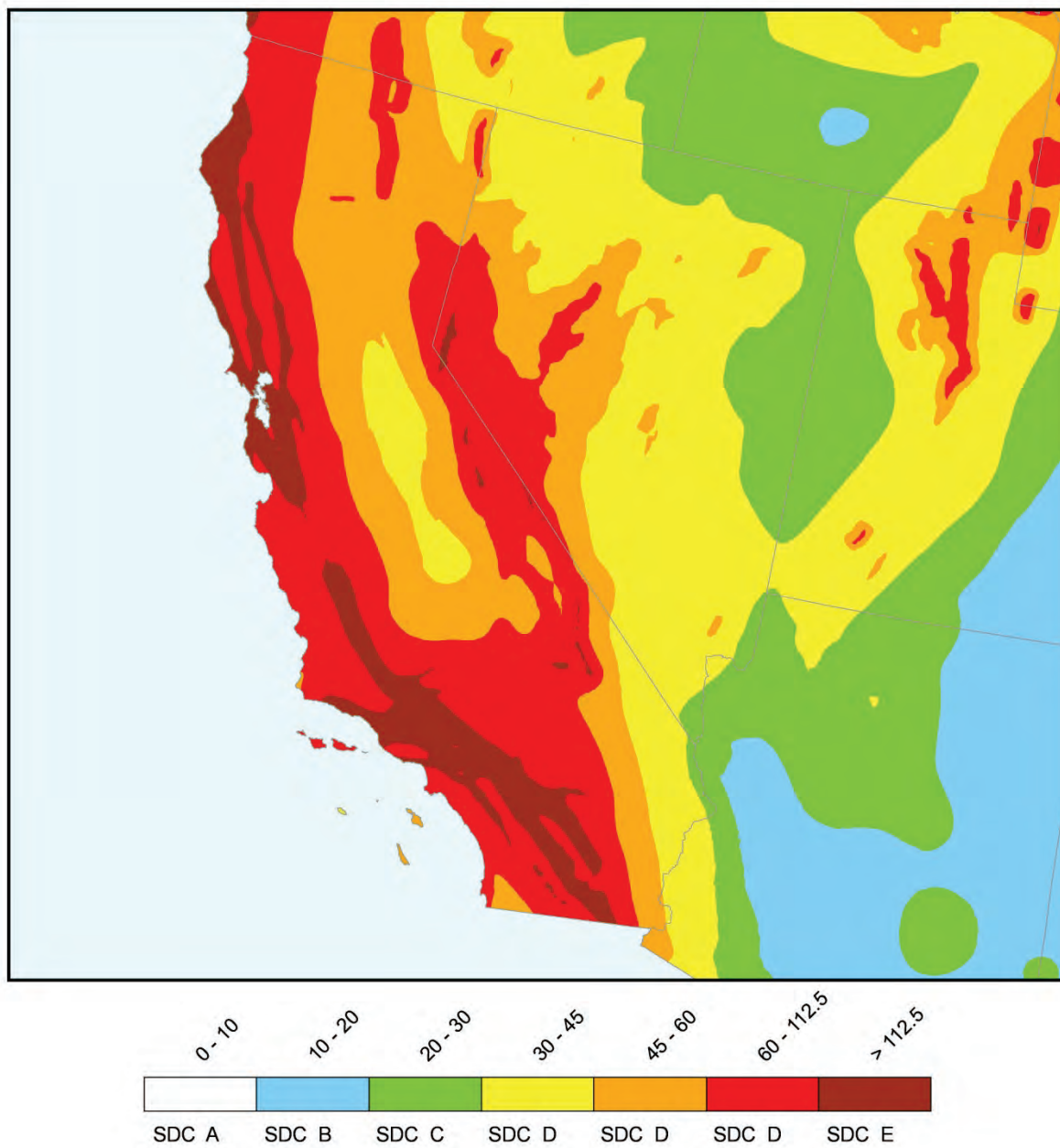
Figure C11.4-3 Map illustrating values of the MCE_R 1-second spectral response acceleration parameter, S_{M1} (%g), and associated regions of Seismic Design Category, assuming Site Class D conditions, for California sites.
