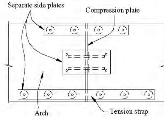
Figure C1.1.3 Typical arch moment splice.
